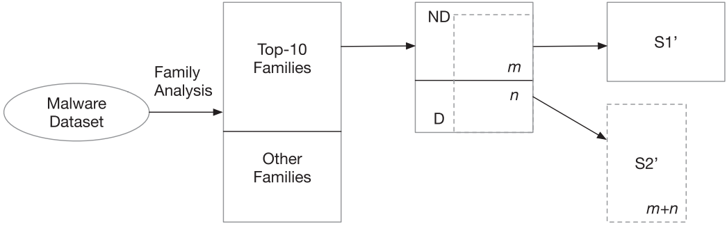
Fig. 11. Training set preparation for ML-based malware family classification.
