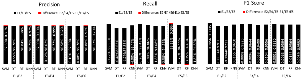
Fig. 9. Experiment results with different ML algorithms on AMD dataset.
