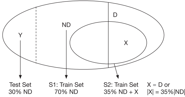
Fig. 6. The experiment design of ML-based Malware Detection. X stands for the set of samples selected from |D| , while Y stands for the set of apps selected for fulfilling the test set 6 and prepare the training set in two settings, noted as S1 and S2 in Figure 6.
