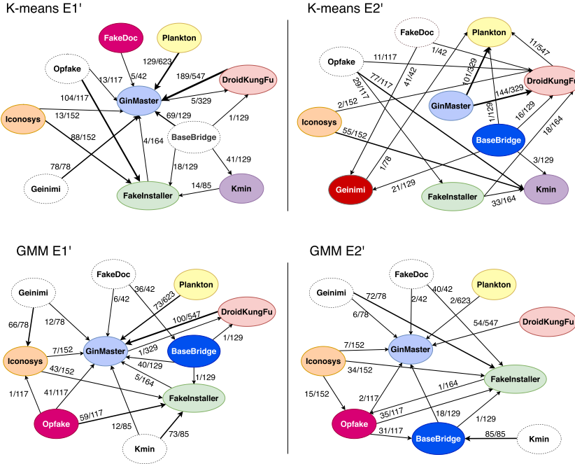
Fig. 12. Visualization of the misclassified malware families (for E1'/E2' of the Drebin dataset). The colored shapes represent the retained families. The shapes with dotted lines represent such families that are not identified by the clustering approach.
